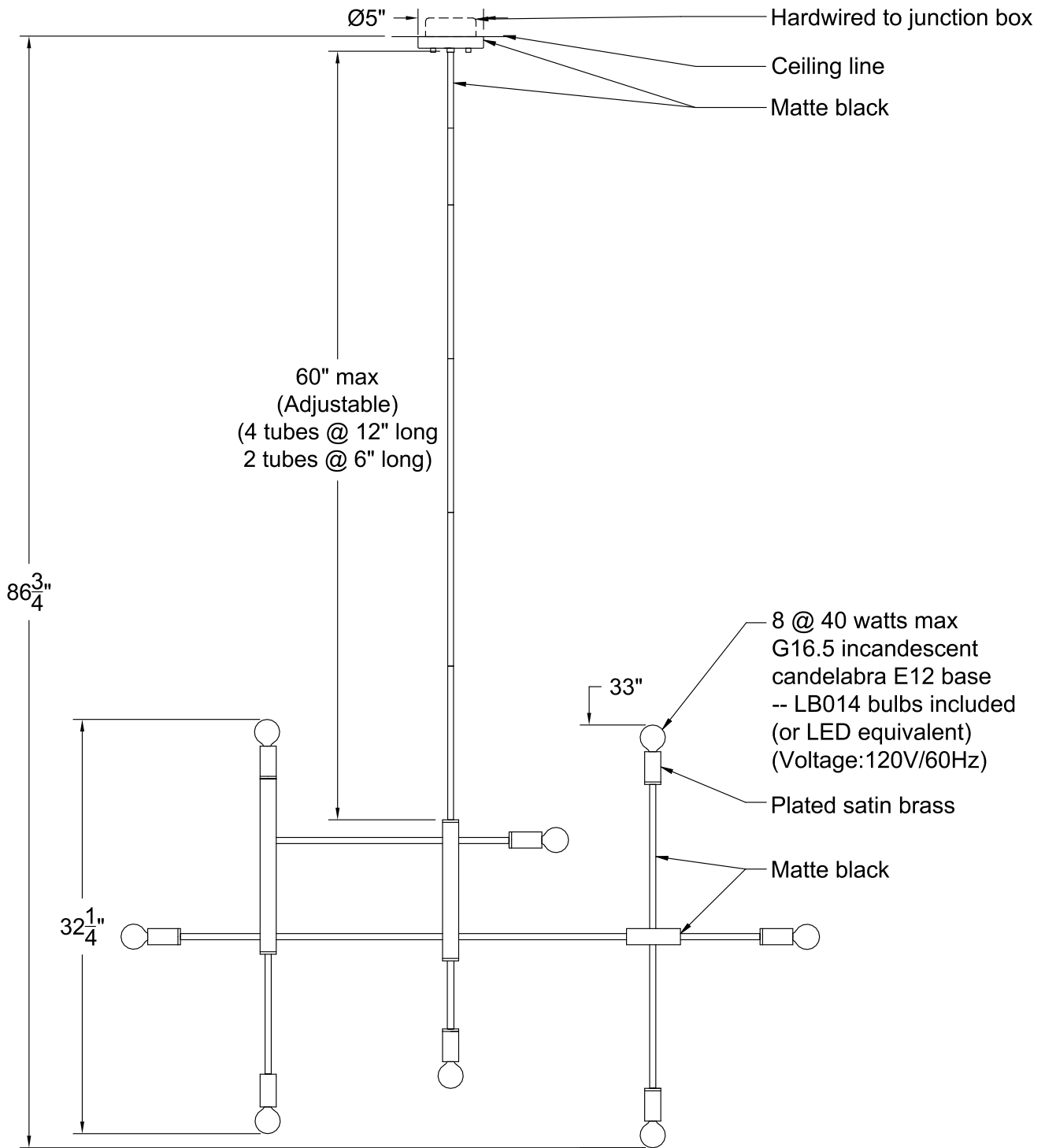
FRONT VIEW
