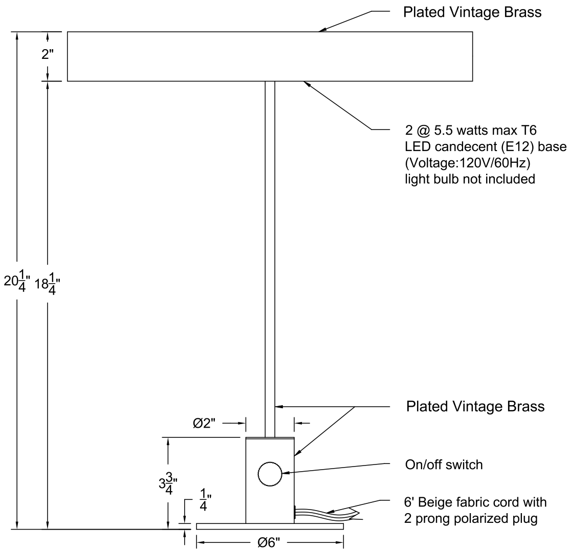
FRONT VIEW
