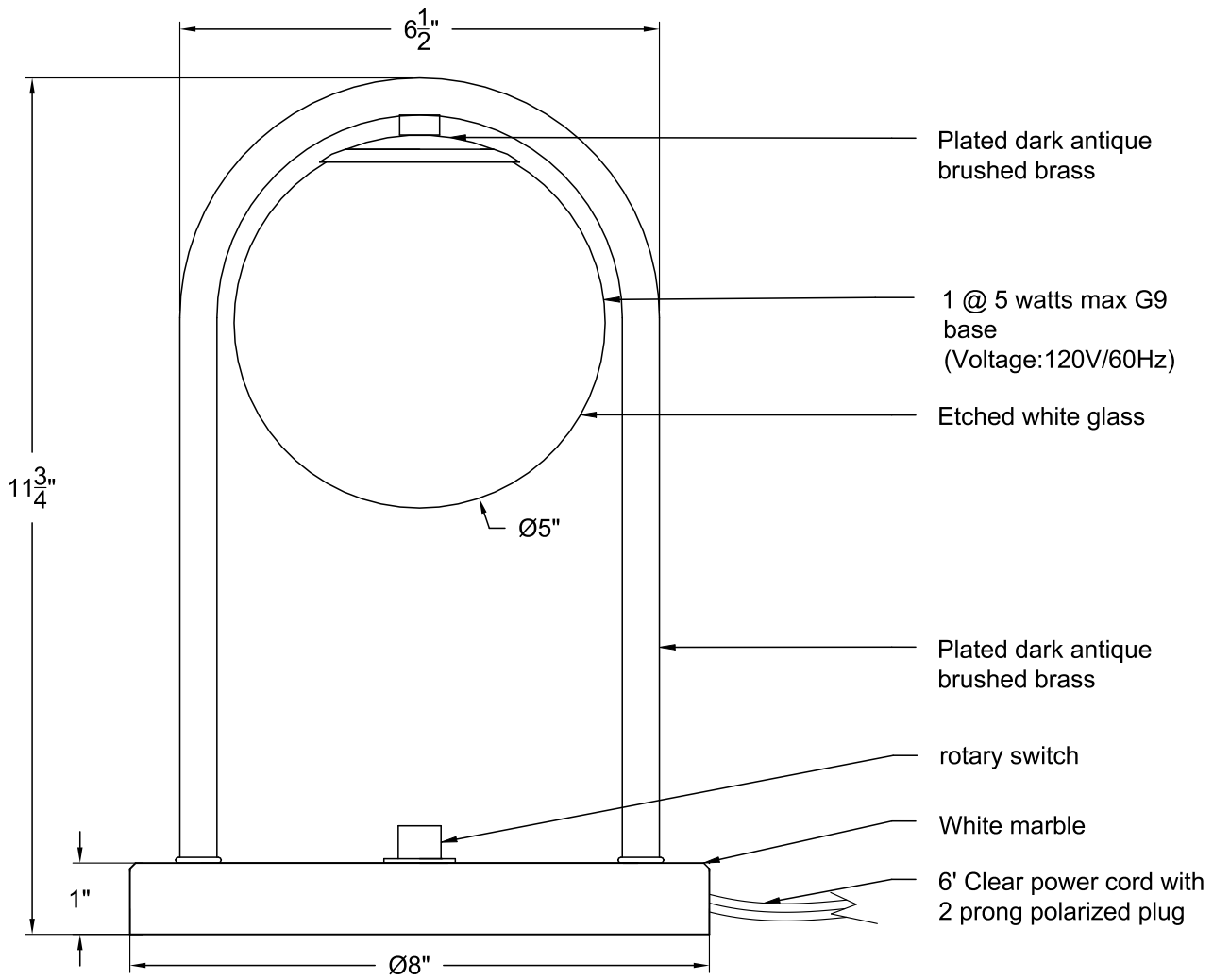
FRONT VIEW
