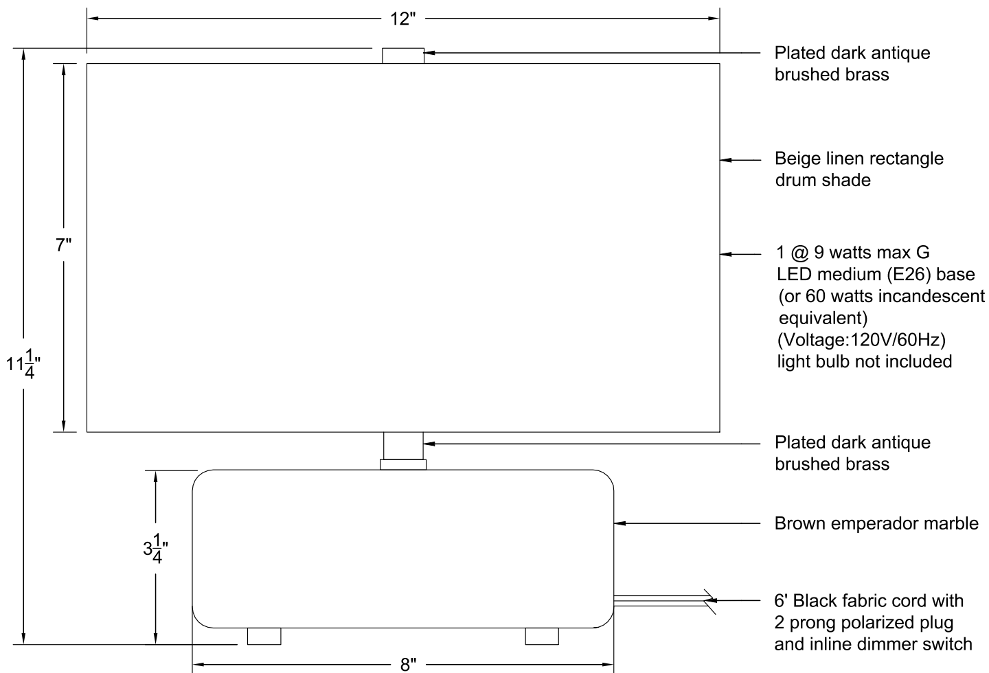
FRONT VIEW
