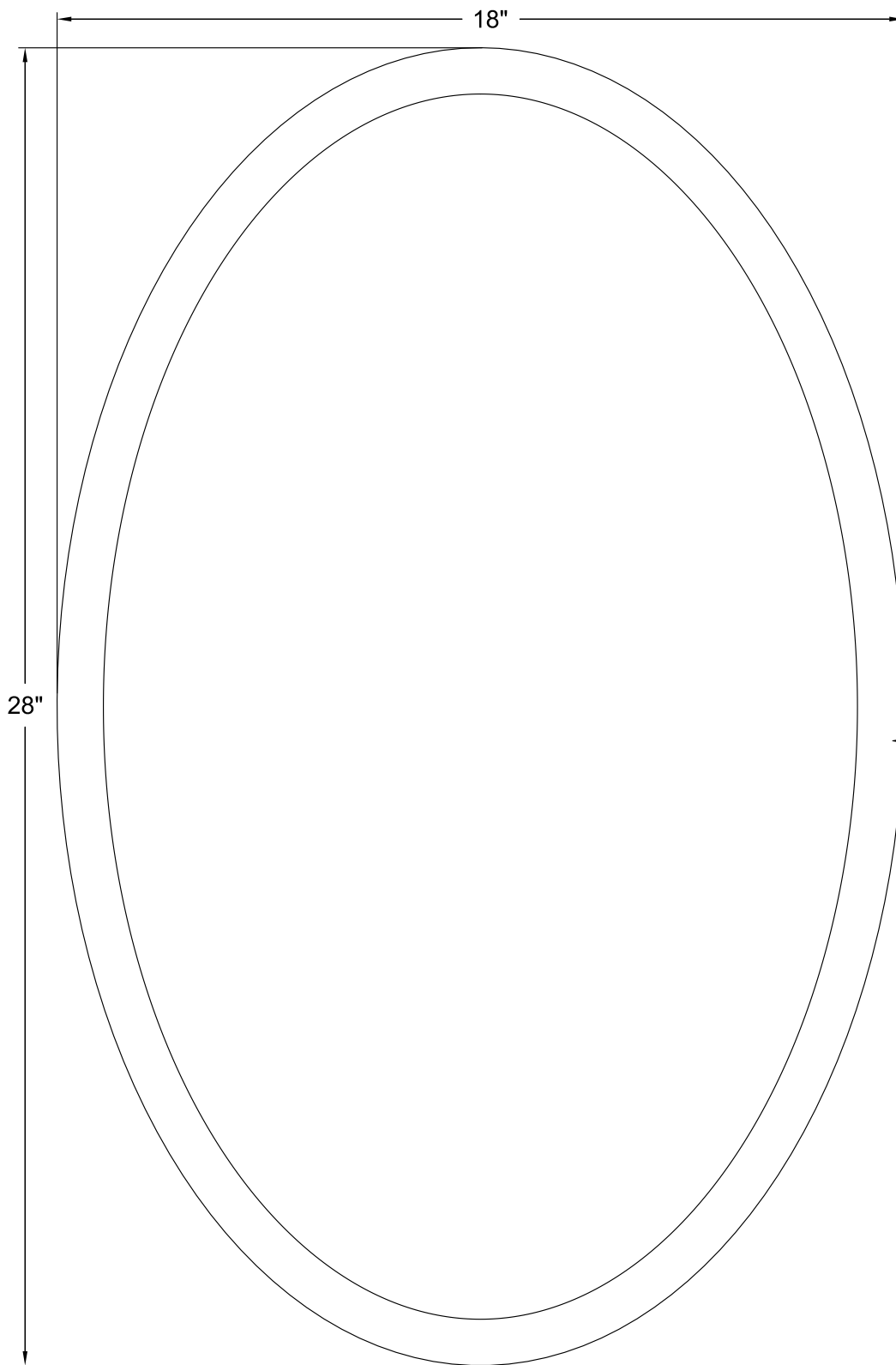
FRONT VIEW
