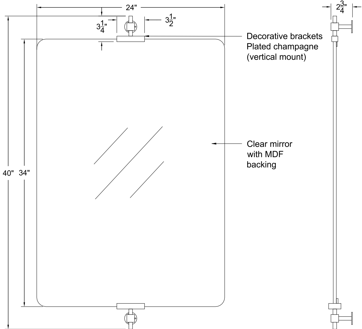
FRONT VIEW
