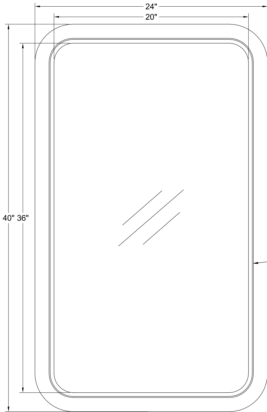
FRONT VIEW
