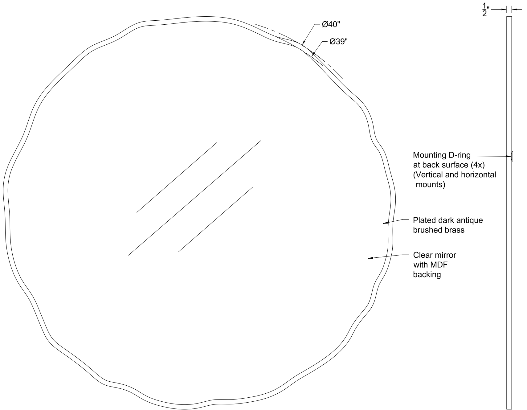
FRONT VIEW
