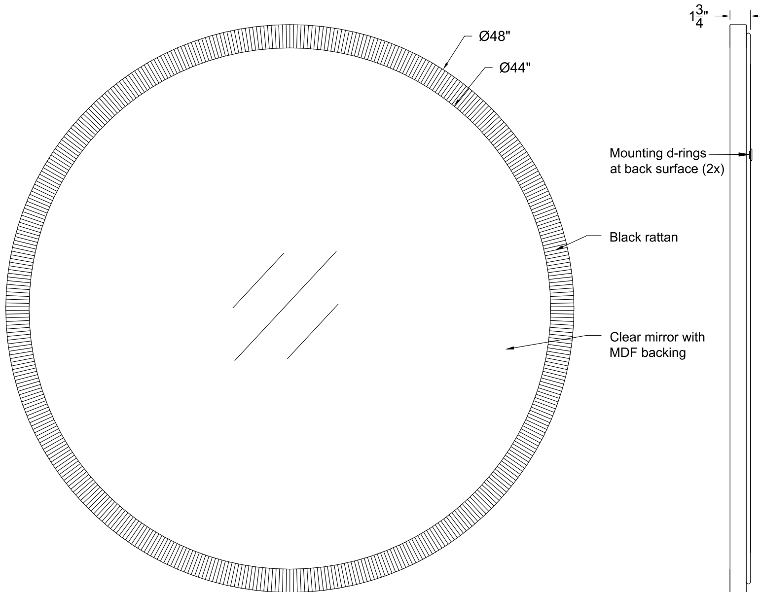
FRONT VIEW
