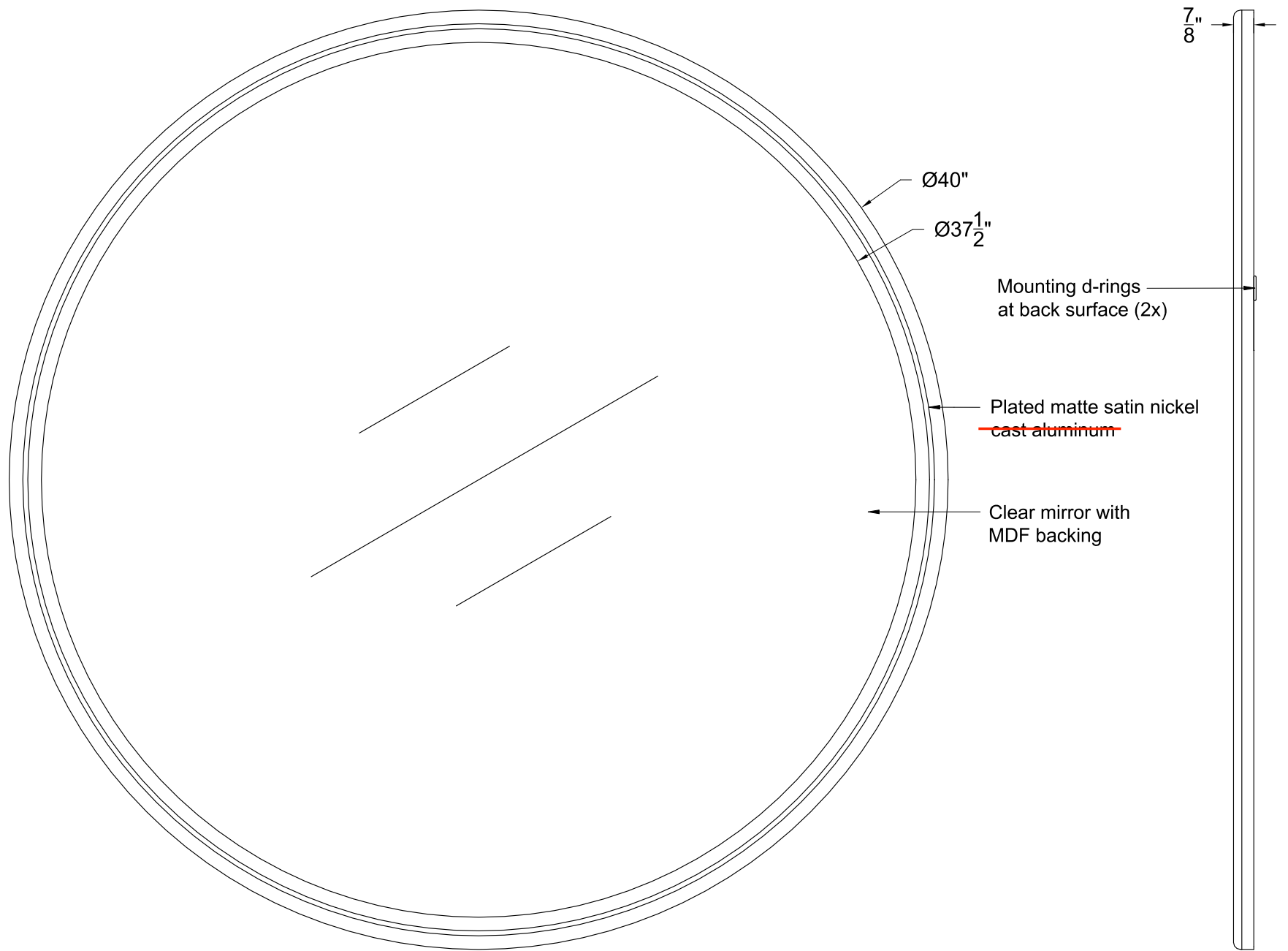
FRONT VIEW
