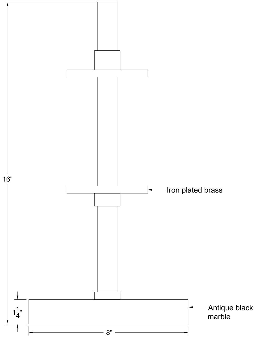
FRONT VIEW
