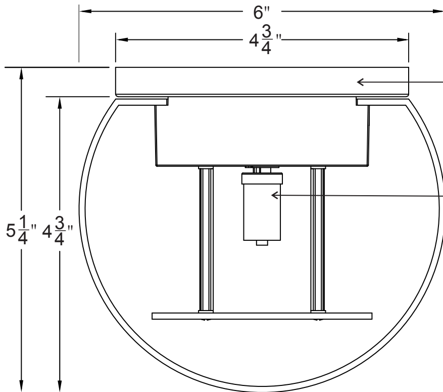
BOTTOM VIEW
