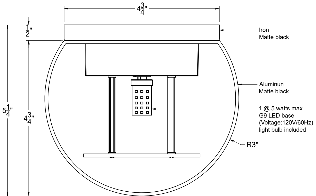
BOTTOM VIEW
