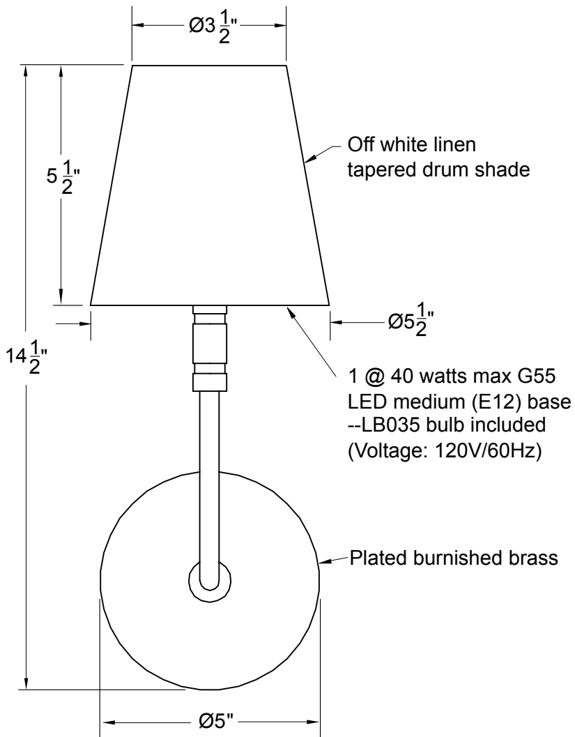
FRONT VIEW
