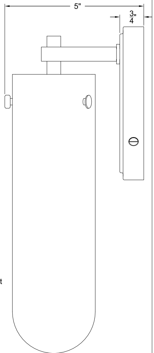
SIDE VIEW
