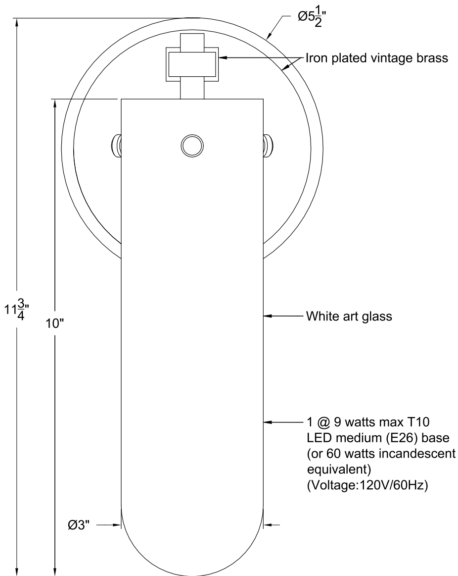
FRONT VIEW
