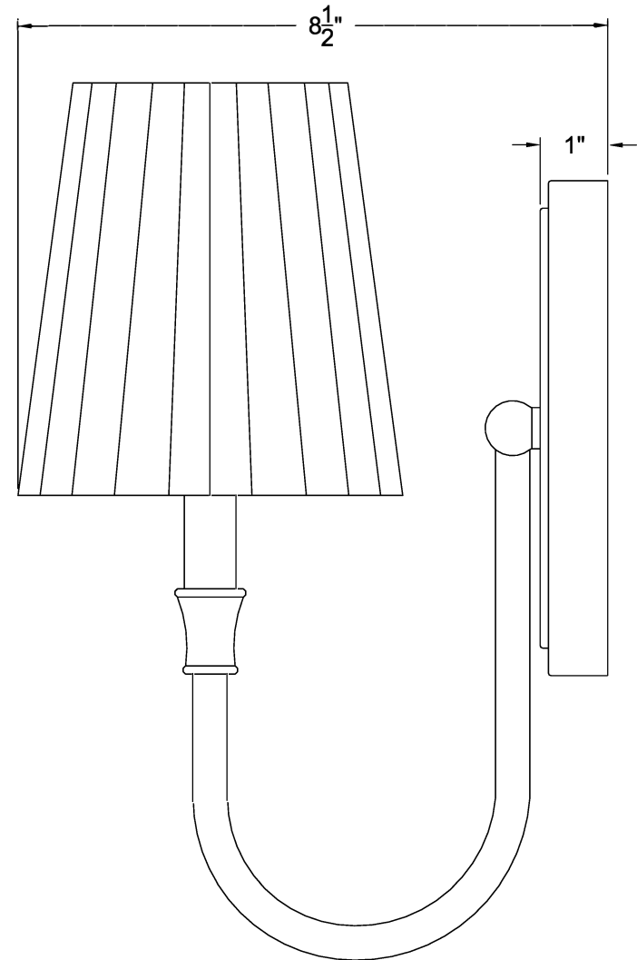
SIDE VIEW
