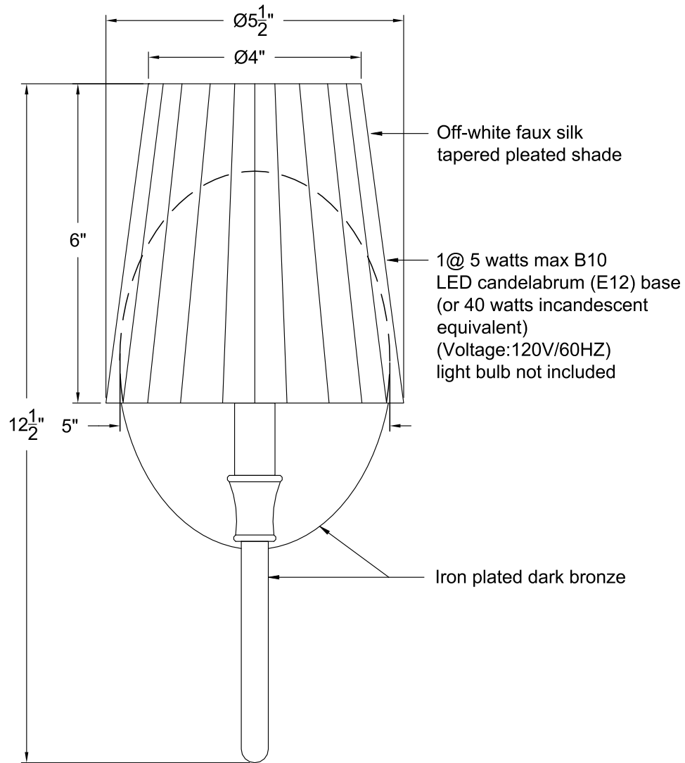
FRONT VIEW
